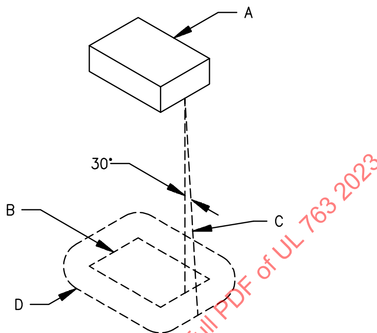
Figure 8.1 Location and extent of barrier
