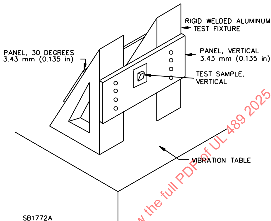
Figure H2.1 Typical vibration-table test setup
