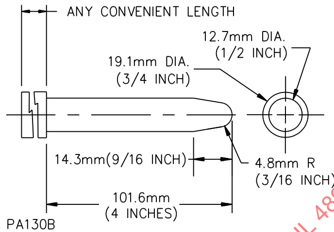
Figure 101.2 Straight probe
