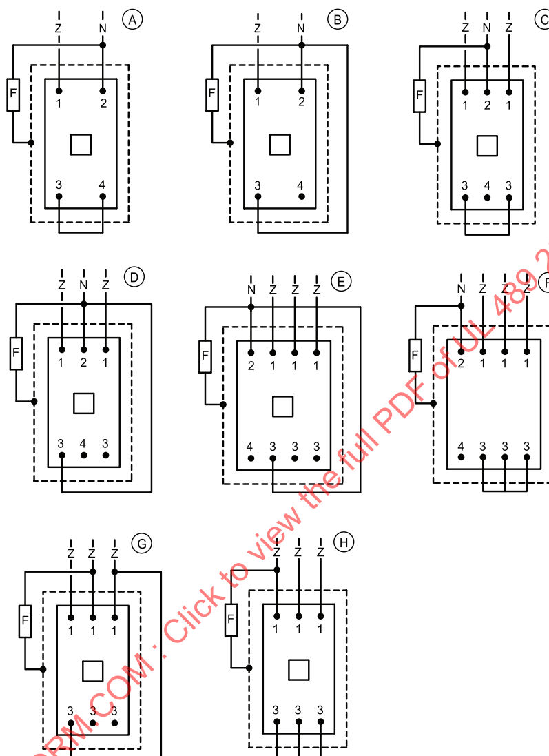
Figure 30.2 Interrupting Test Connections
