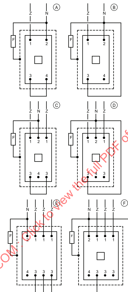
Figure 29.2 Interrupting Test Connections
