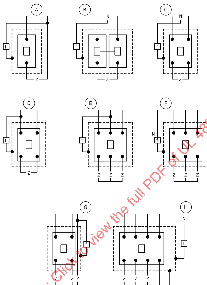
Figure 26.6 Endurance Test Connection Diagrams
