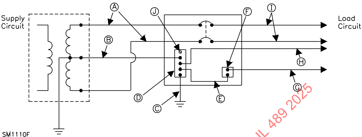
Figure 101.1 Typical Grounding System for Single-Phase Service
