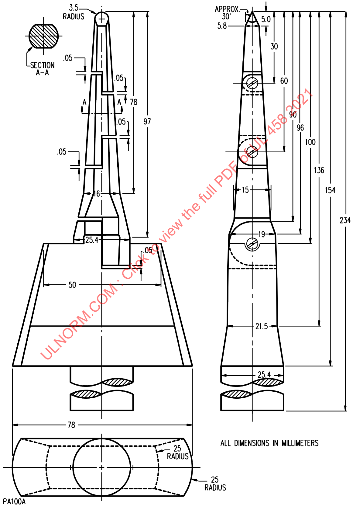
Figure 9.1 Accessibility probe
