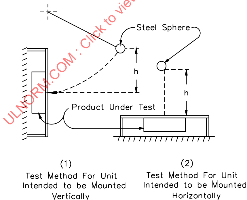
Jarring test
