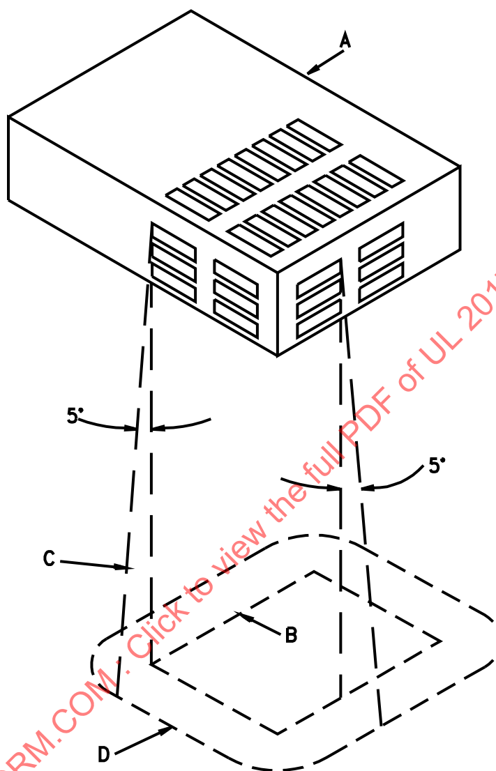
Figure 8.3 Enclosure bottom
