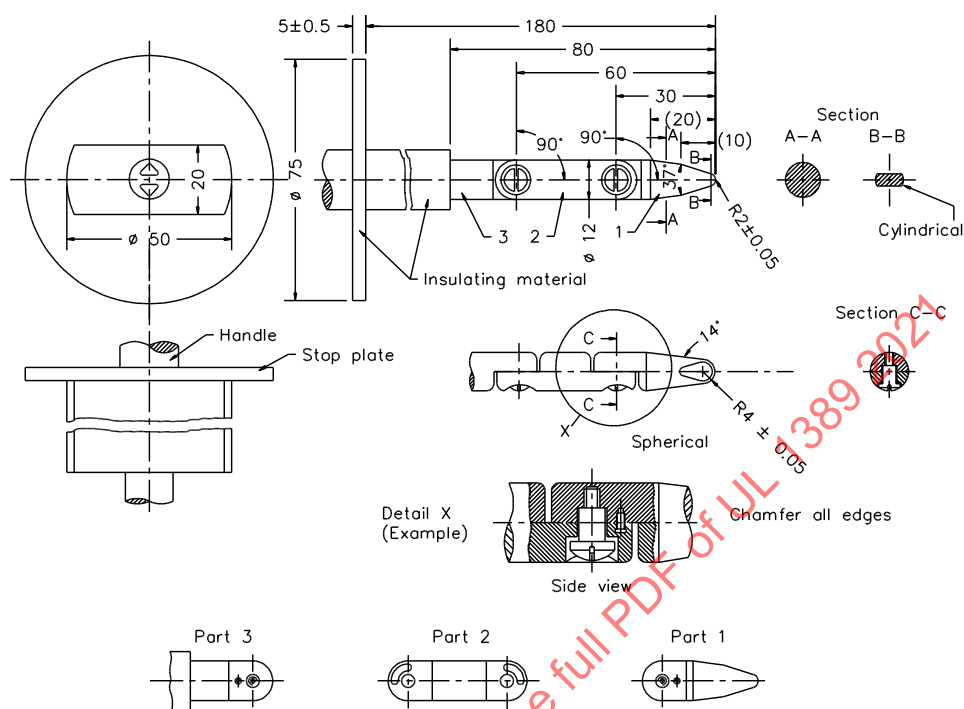
Figure 18E.4 Articulate probe
