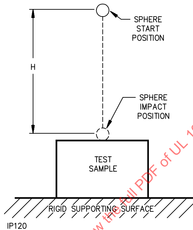
Figure 39.2 Ball drop impact test
