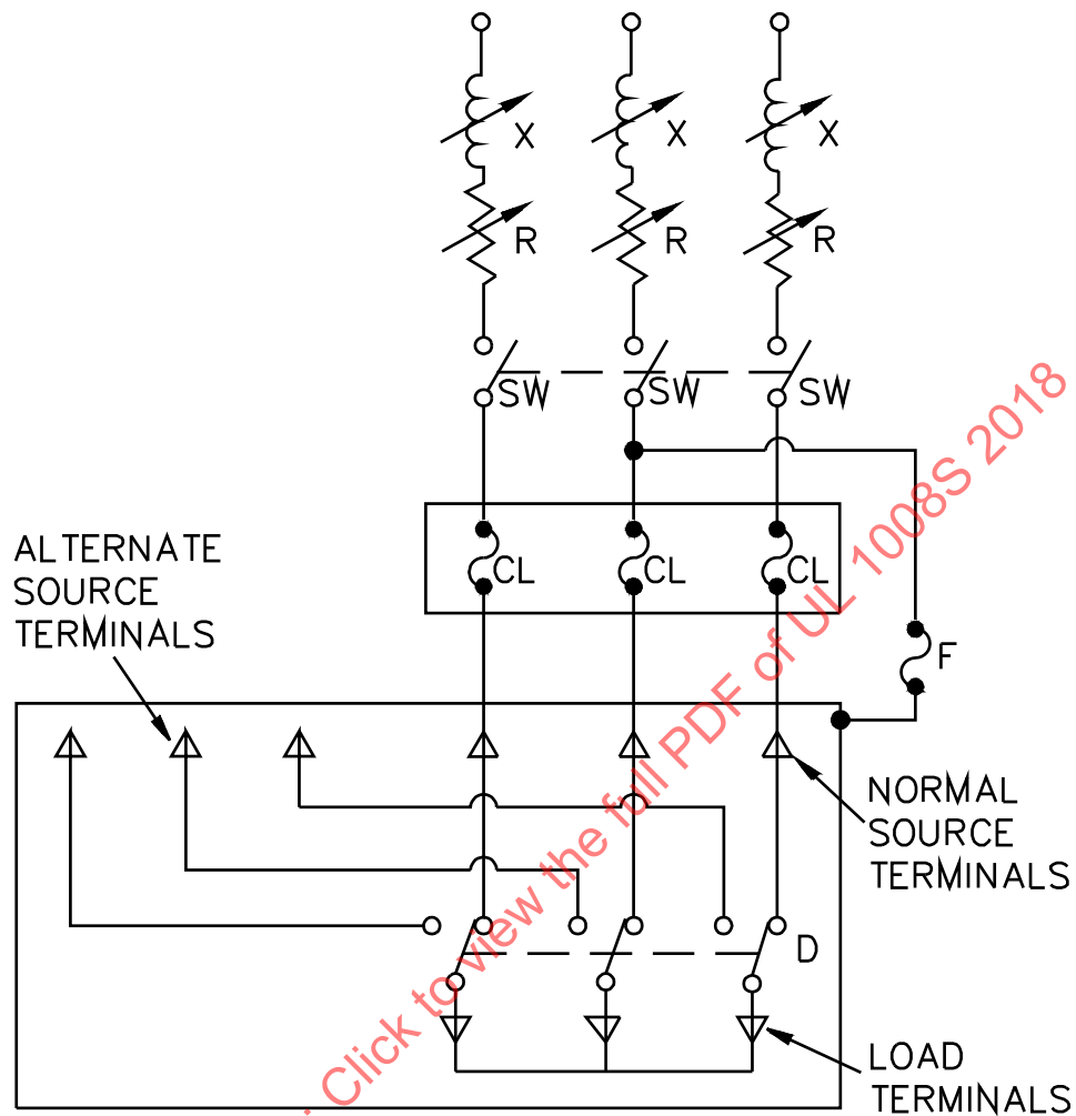
Figure 35.1 Circuit for withstand and closing tests
