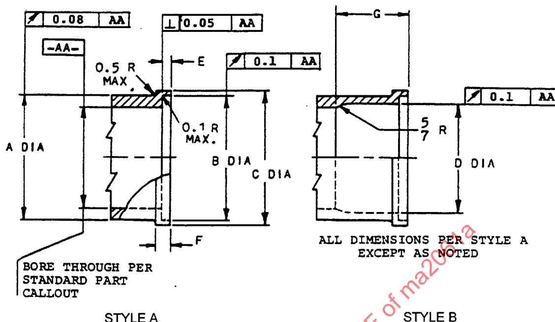
FIGURE 1 - FITTING END
