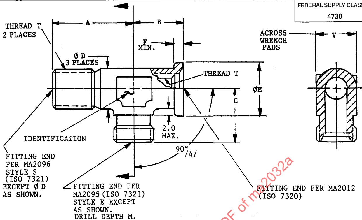
FIGURE 1 - FRONT AND SIDE VIEWS
