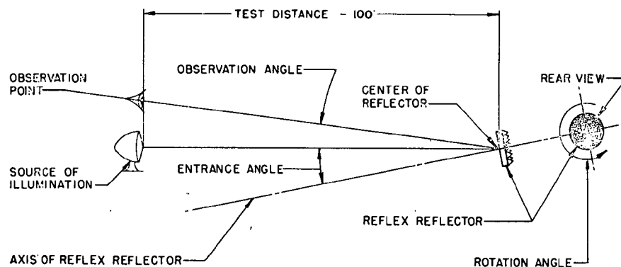
FIG. 1—SETUP FOR TESTING
