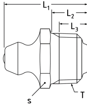
Figure 6 - Straight fittings
