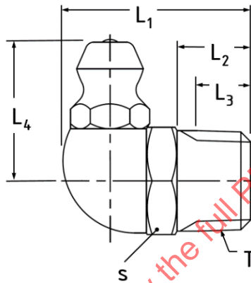
Figure 7 - 90 Degree elbow fittings
