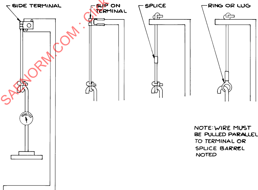
FIGURE 1—EXAMPLES OF SOME TERMINAL PULL-OFF METHODS
