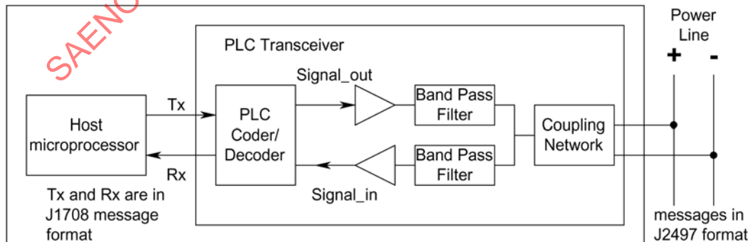
FIGURE 2—PLC TRANSCEIVER
