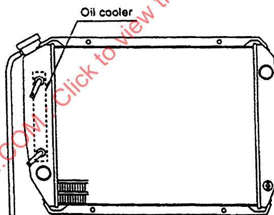
FIGURE 3—EXAMPLE OF OIL COOLER INSTALLATION (CROSSFLOW TYPE RADIATOR)
