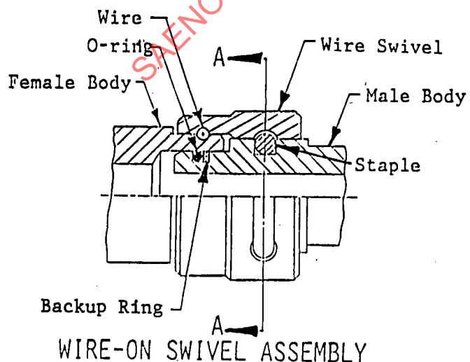
FIGURE 1 - Typical Assemblies of Swivel and Fixed Connections
