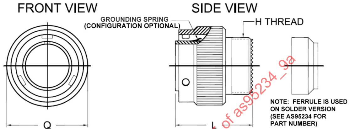
FIGURE 1 - CONNECTOR PLUG, GROUNDING
