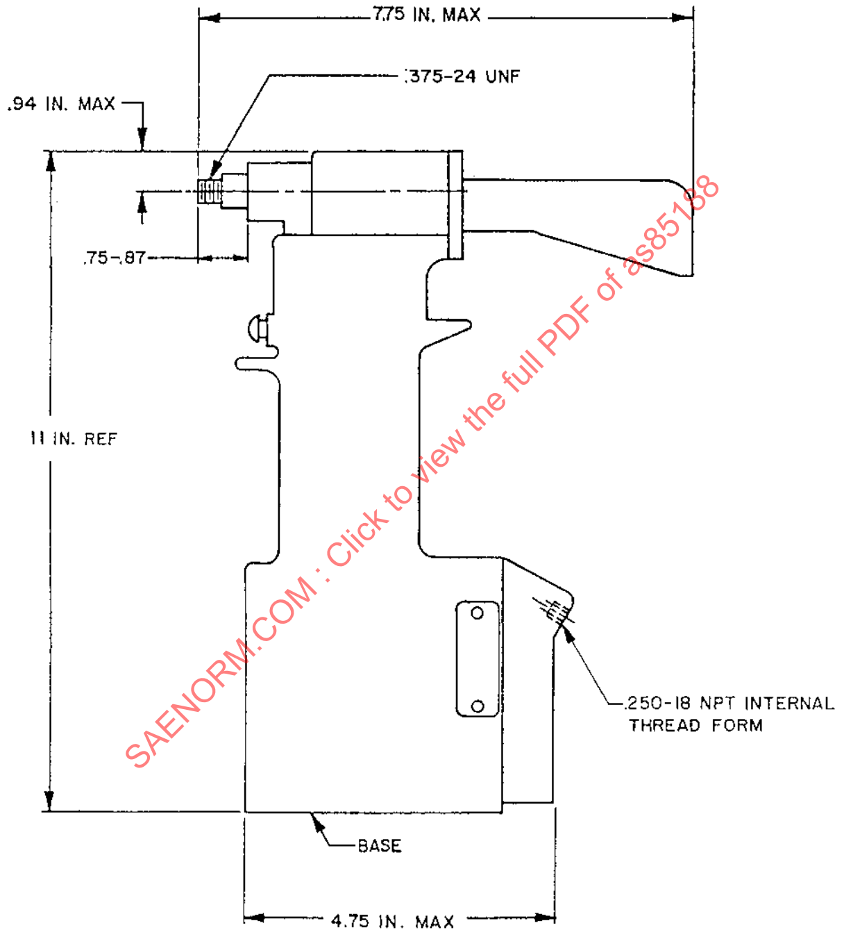
FIGURE 2. Riveter, Type 1
