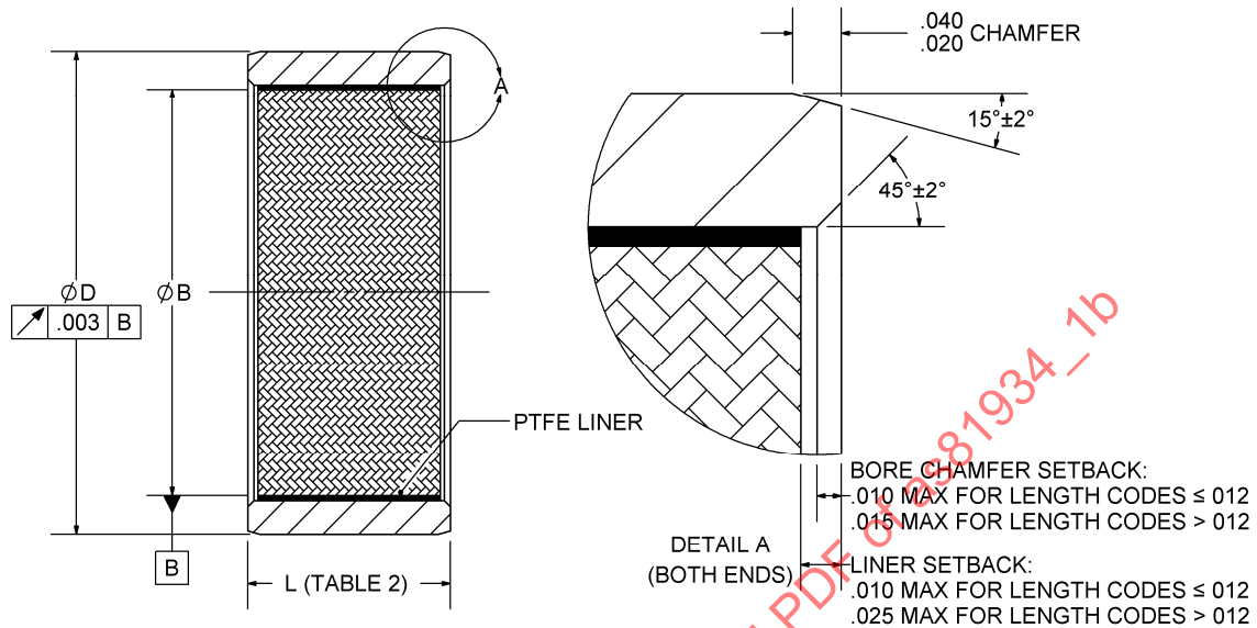
FIGURE 1 - PART CONFIGURATION
