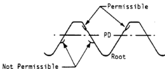
FIGURE 7 - Laps Extending Towards Crest, Rolled Thread
