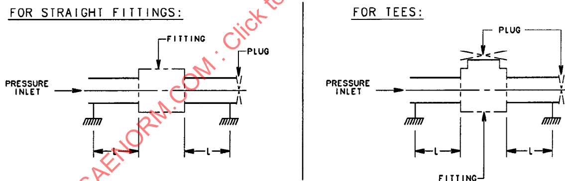
FIGURE 6 - VIBRATION TEST SETUP
