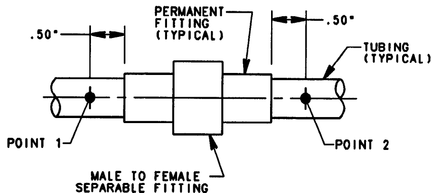
FIGURE 5 - FITTING CONDUCTIVITY
