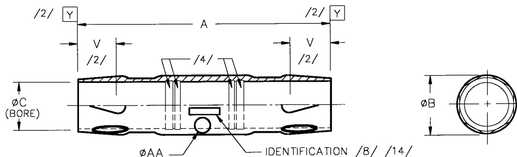
FIGURE 1 - UNION, EXTERNAL SWAGE
