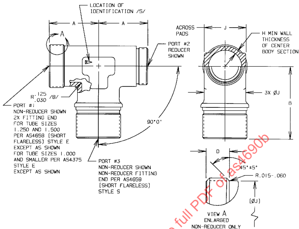
FIGURE 1 - FITTING, TEE, REDUCER
