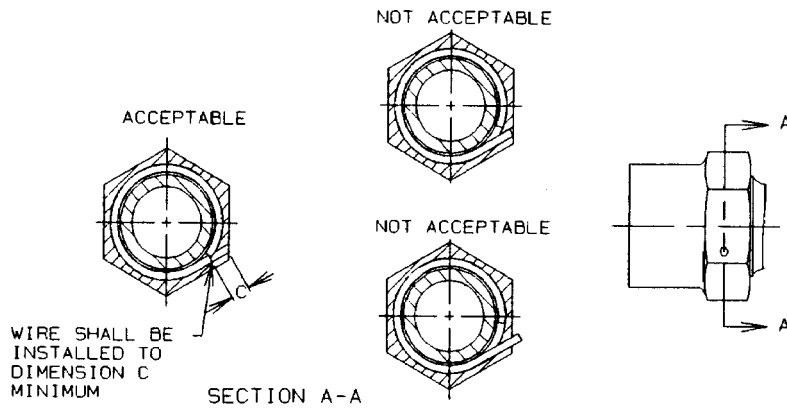
FIGURE 2 - INSTALLATION, SWIVEL NUT RETAINING WIRE
