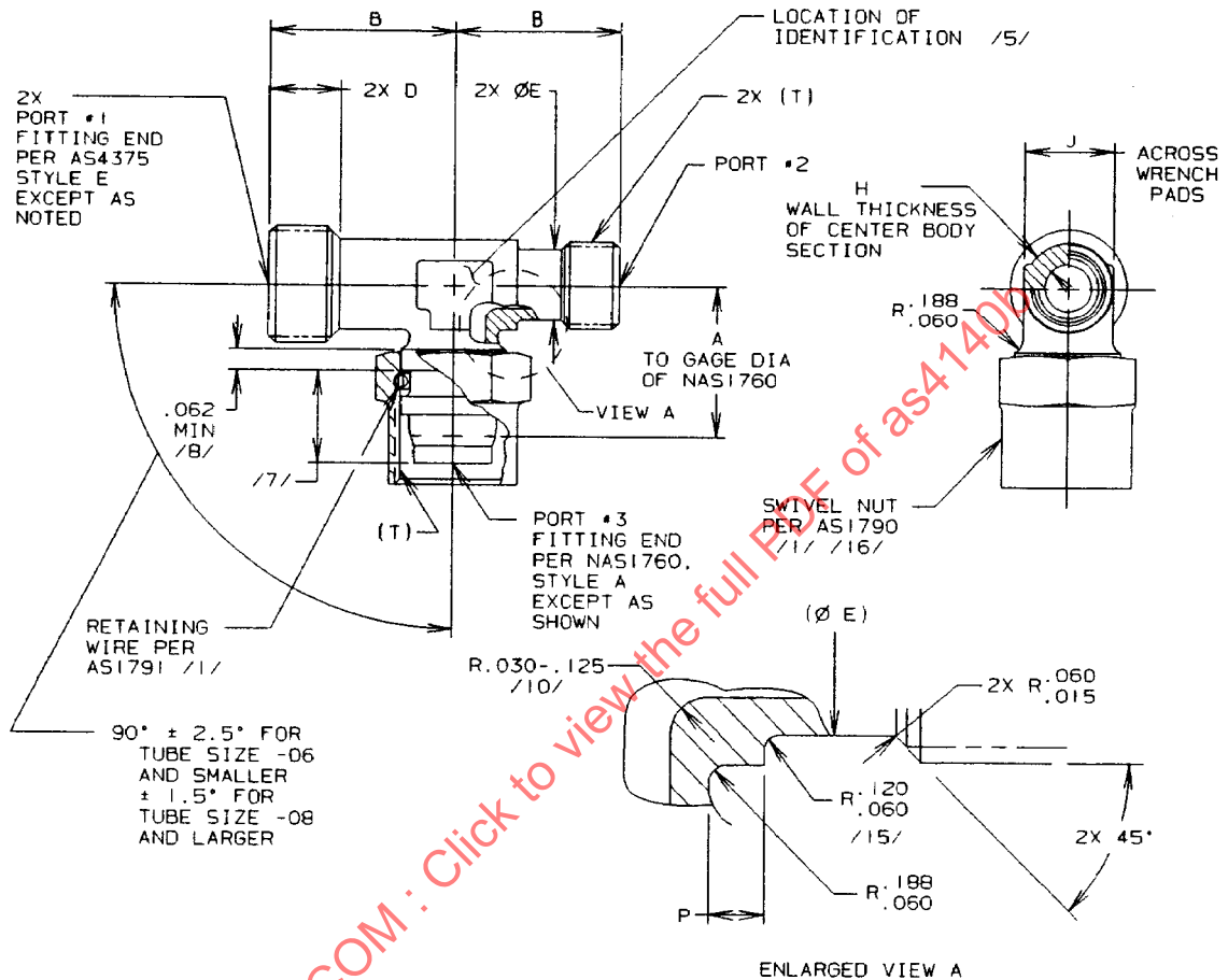
FIGURE 1 - FITTING ASSY, TEE, REDUCER, SWIVEL ON SIDE, REDUCED BODY, FLARELESS
