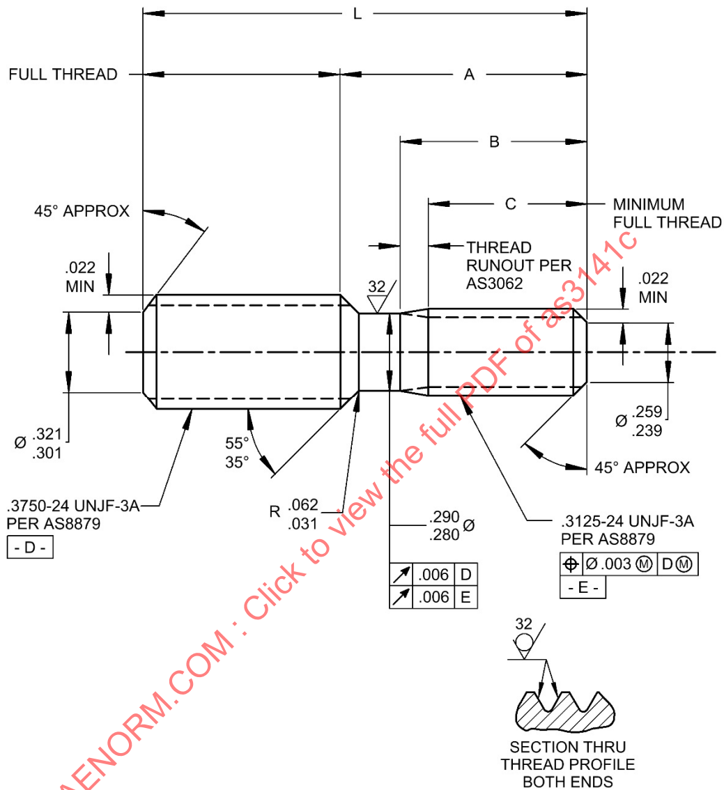
FIGURE 1 - STUD
