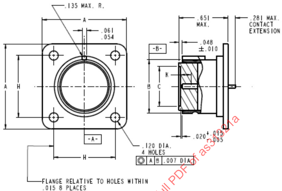
STYLE S (SOCKET INSERT)
