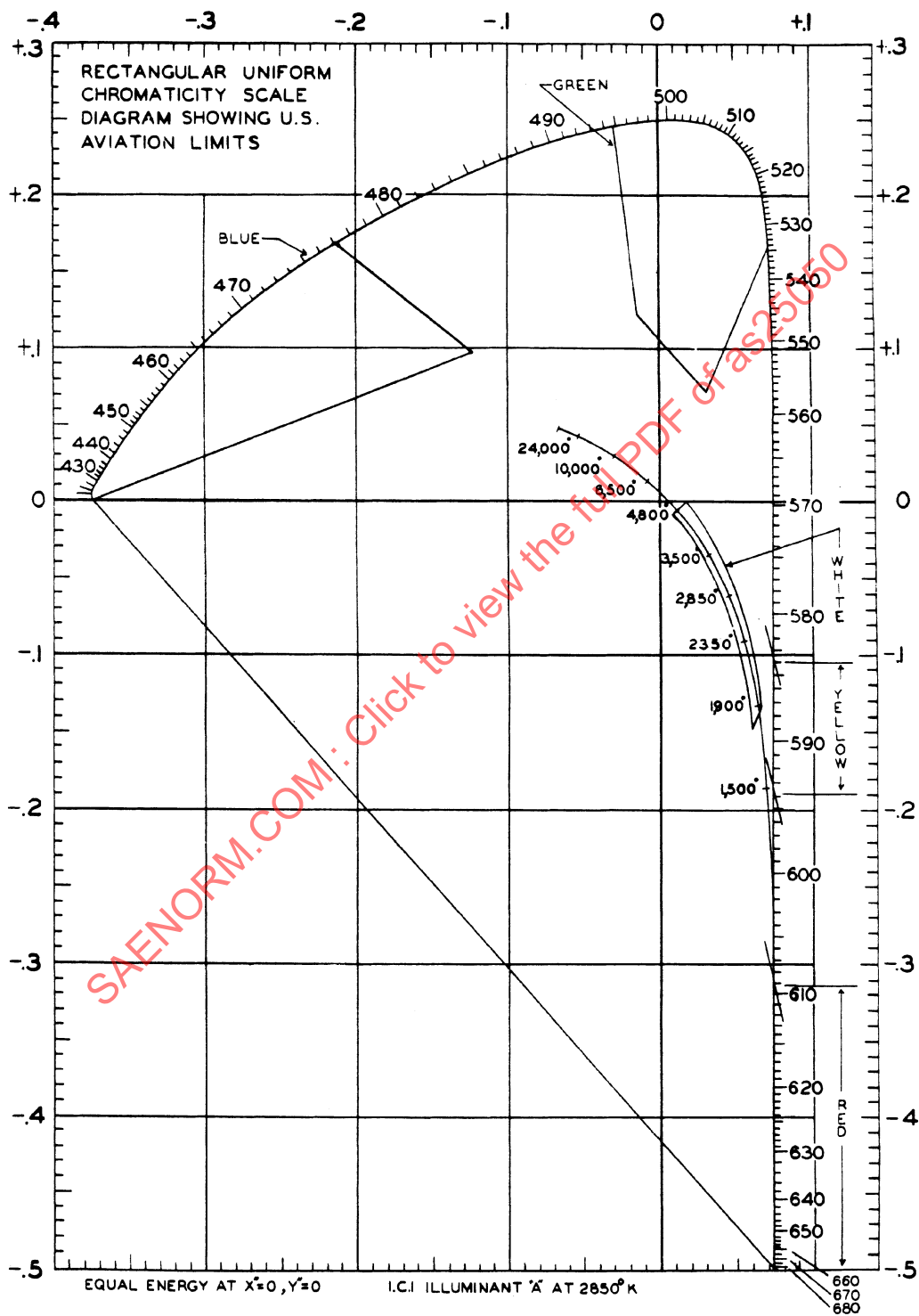
FIGURE 3. R.U.C.S. Mixture diagram showing aviation color limits
