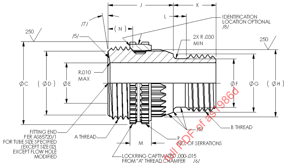
FIGURE 1 – ADAPTER, ASSEMBLY
