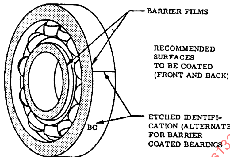
DETAIL A - UNFLANGED BEARING
