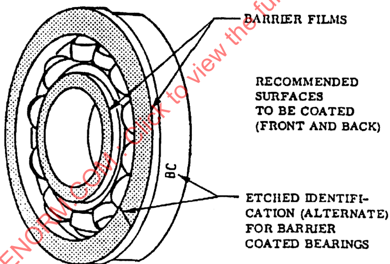
DETAIL B - FLANGED BEARING
