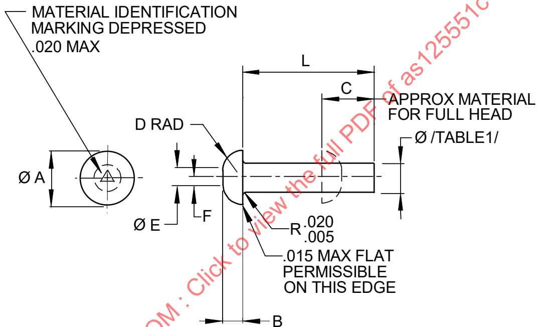
FIGURE 1 - RIVET
