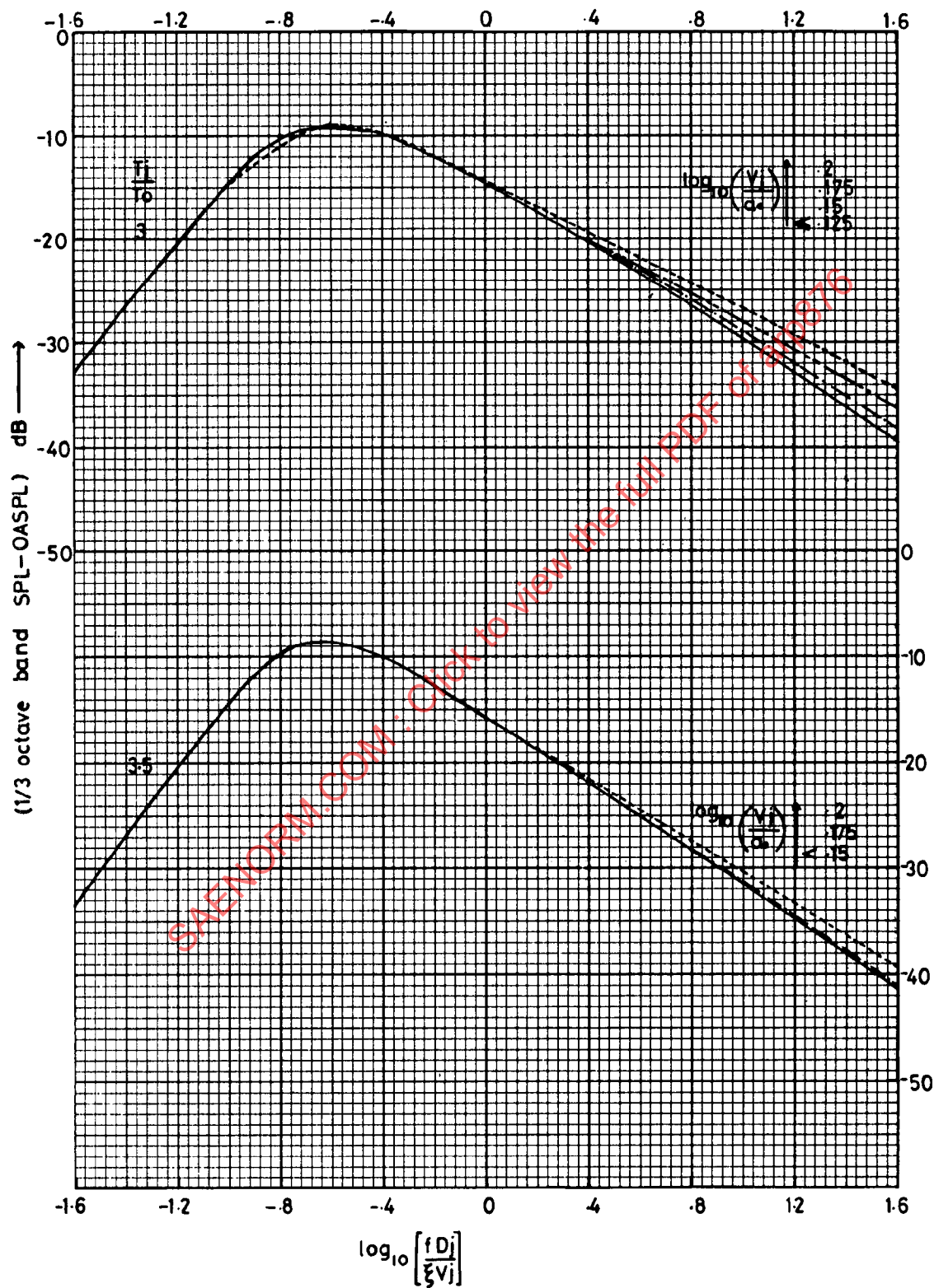
FIG. A8. (CONT'D) 1/3 OCTAVE BAND NORMALISED SPECTRA. O_i = 130^\circ
