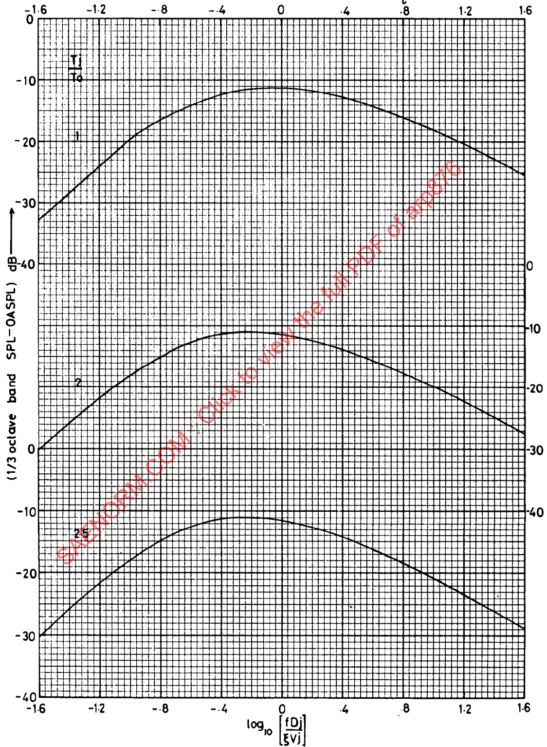
FIG. A4. 1/3 OCTAVE BAND NORMALISED SPECTRA. \theta_i \leq 90^\circ
