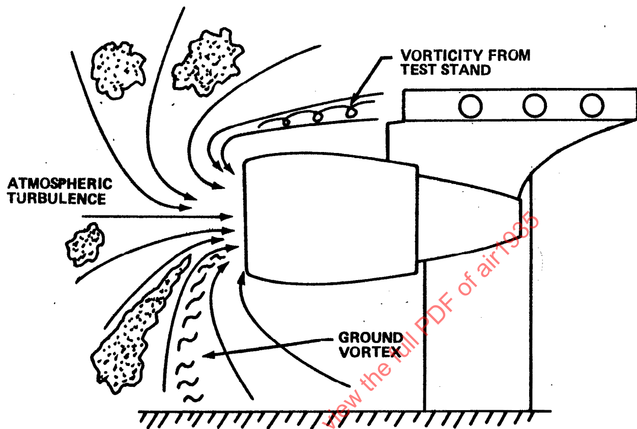
(a) GROUND STATIC TEST
