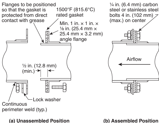
Δ FIGURE 8.1.3.2(b) Typical Section of Duct-to-Fan Connection — Overlapping Method.
