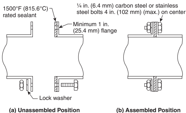
Δ FIGURE 8.1.3.2(c) Typical Section of Duct-to-Fan Connection — Sealant Method.
