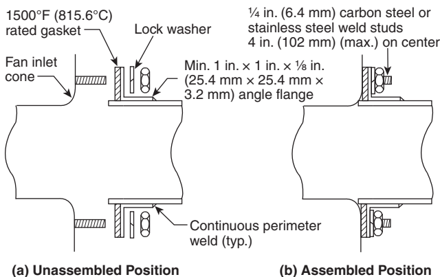
Δ FIGURE 8.1.3.2(d) Typical Section of Duct-to-Fan Connection — Direct to Fan Inlet Cone Method.
