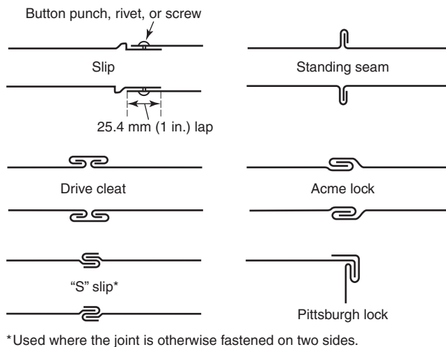
FIGURE 4.3.2.3 Types of Duct Joints.
