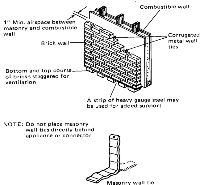
Figure 3-1.4(c) Masonry clearance reduction system.
