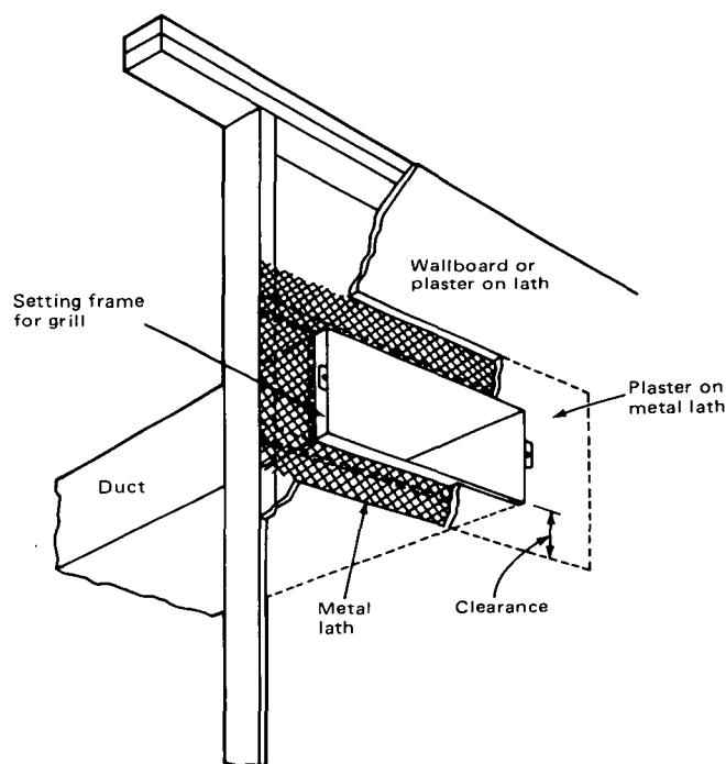
Figure 3-1.2(a) An arrangement for closing ends of clearance space around a supply duct. A similar arrangement can be used where a duct continues on through the partition.
