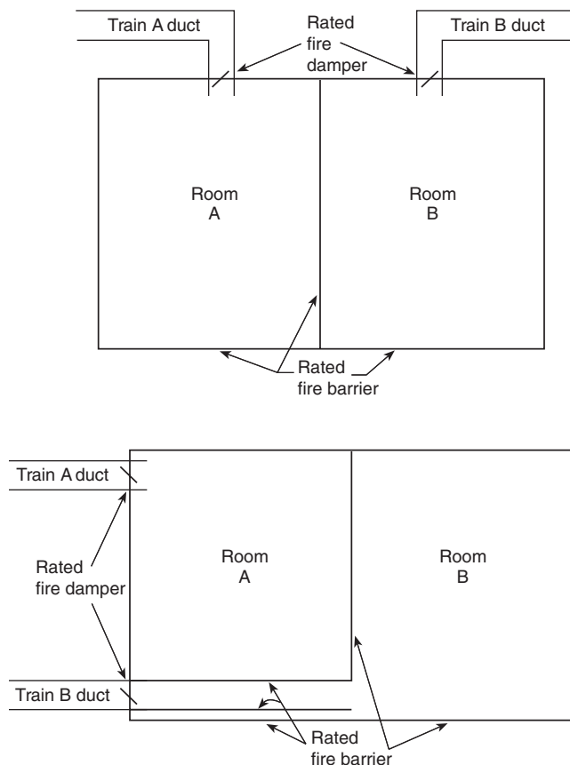
FIGURE A.8.4.8.2 Typical Air Duct Fire Damper Configuration.
