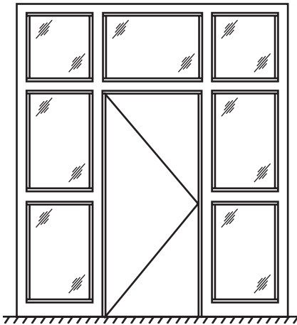
FIGURE A.3.3.52(c) Transom and Side Light Frame.
