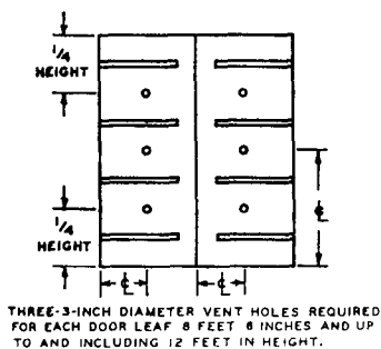
Figure A-33. Location of vent holes for swinging doors.
