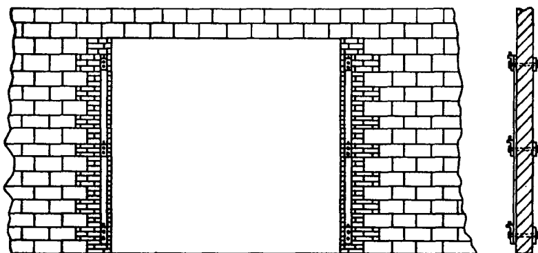
Figure A-16. Concrete block wall prepared for doors swinging in pairs — lap mounted, standard method.
