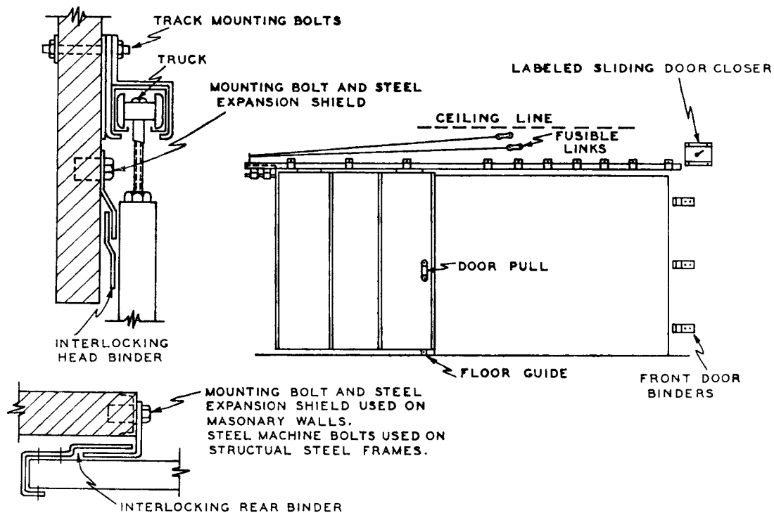
Figure A-43. Horizontally sliding hollow metal door.
