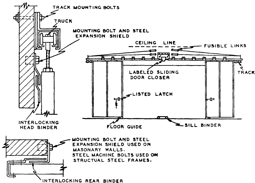
Figure A-44. Center parting horizontally sliding hollow metal doors.
