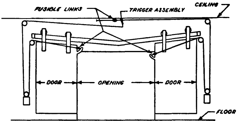
Figure A-38. Closing devices for center parting horizontally sliding doors (inclined track.)
