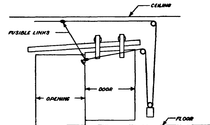
Figure A-35. Closing devices for single sliding door (inclined track.)
