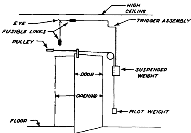
Figure A-30. Closing devices for single swinging door.
