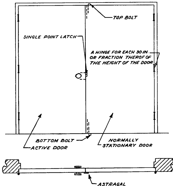
Figure A-21. Builders hardware (doors swinging in pairs with single point latch — flush mounted.)
