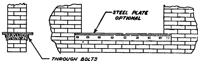
Figure A-3. Angle iron and concrete sill used with combustible floors.
