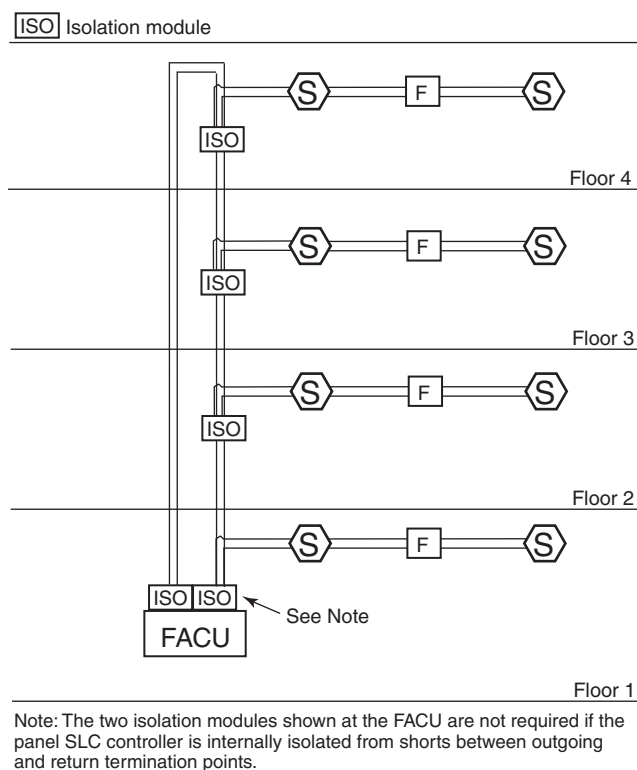
FIGURE A.23.6.1(c) Hybrid Isolation Method.
