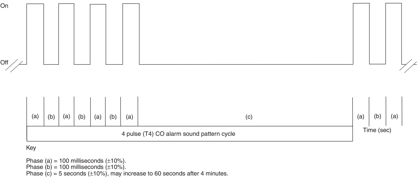
N FIGURE A.29.5.3 Four Pulse Temporal Pattern.
