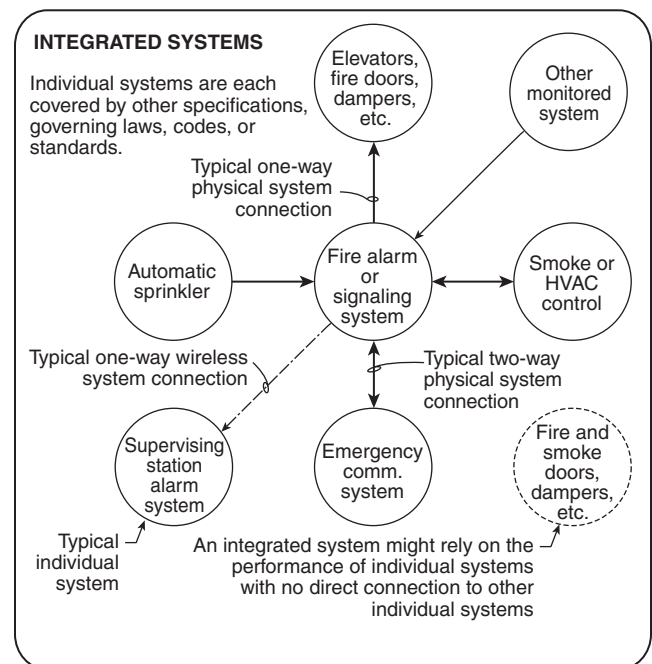
▲ FIGURE A.21.1 Integrated Systems. (Courtesy of R.P. Schiffliti Associates, Inc.)
