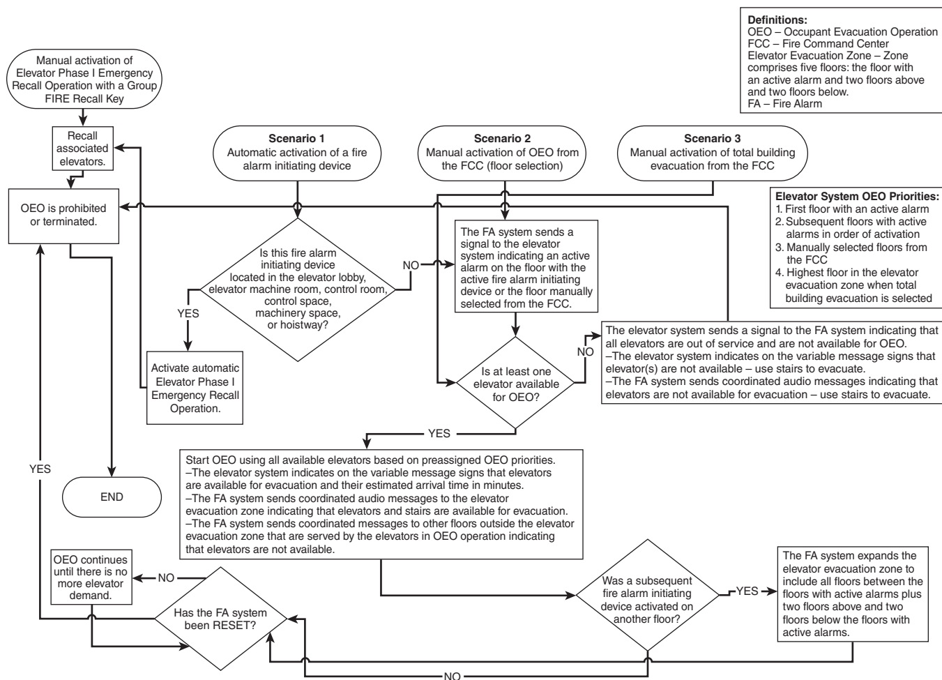
N FIGURE A.21.6 Simplified Occupant Evacuation Operation (OEO) (Elevator system interface with the building fire alarm system based on ASME A17.1, Section 2.27.11, and NFPA 72, Section 21.6).
