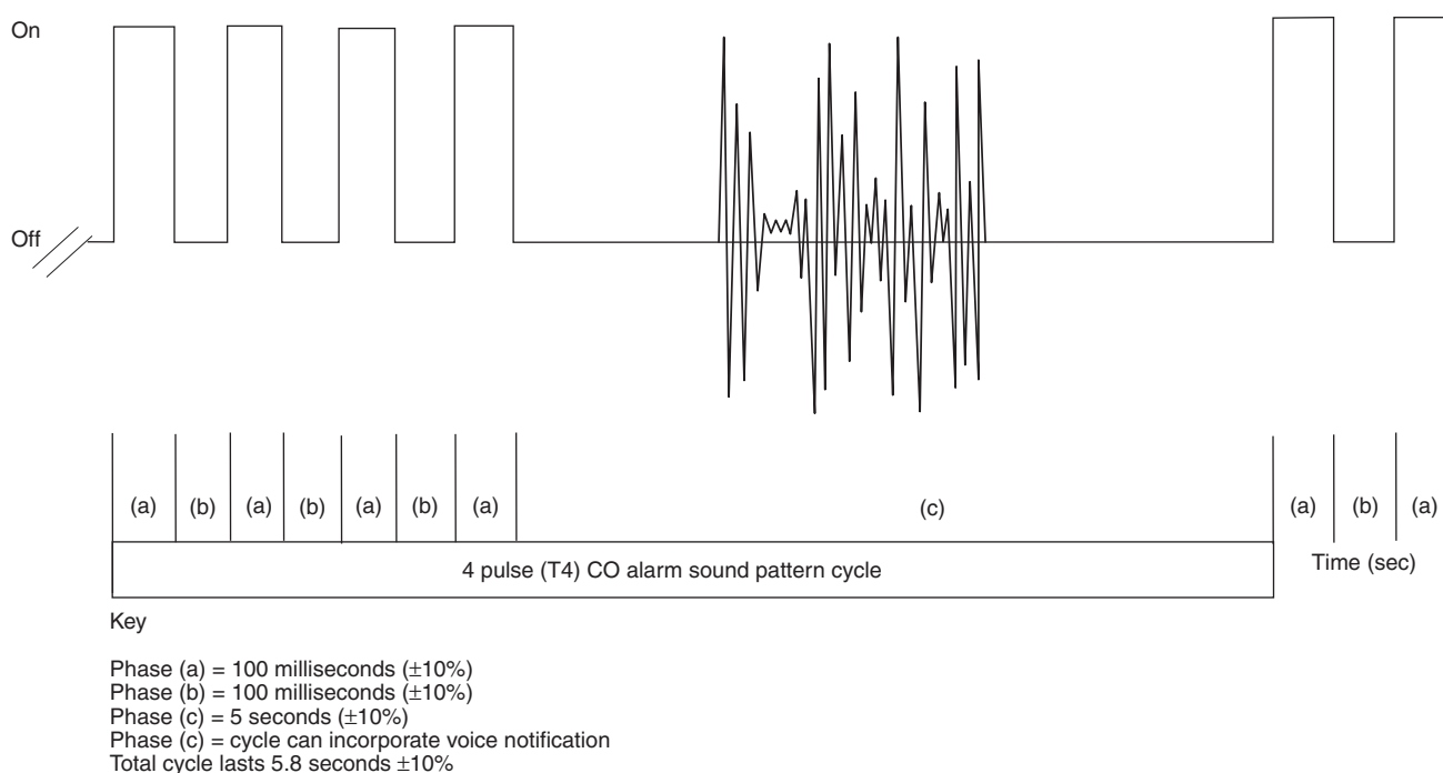
N FIGURE A.29.5.6(b) Temporal Pattern Parameters with 1.5-second Voice Allowance.
