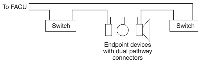
FIGURE A.12.3.6(5) Class N Pathway Block Diagram with Daisy-Chain Devices with Dual Pathway Connection.
