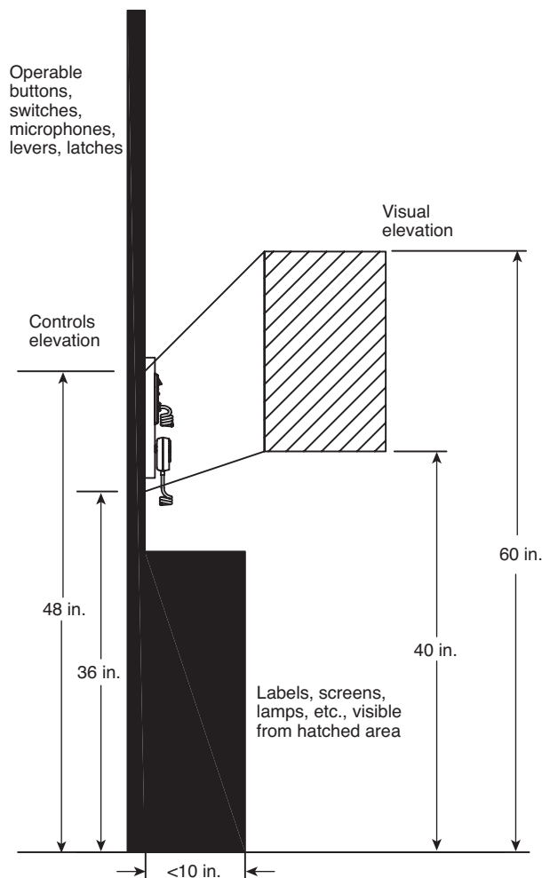
FIGURE A.24.5.14(a) Horizontal Reach of Less Than 10 in. (25 cm).
