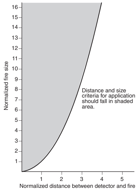
FIGURE A.17.8.3.1 Normalized Fire Size vs. Distance.
