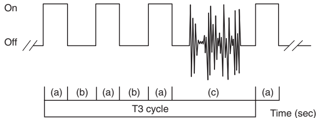
FIGURE A.29.3.5.2(a) Temporal Pattern Parameters with 10-Second Voice Allowance.
