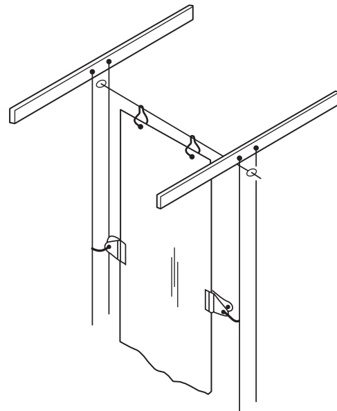
Figure 11-1.2 Test sample flat sheet.
