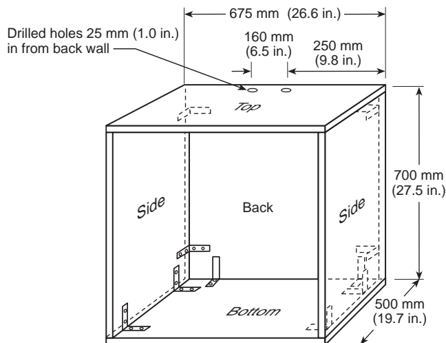
Figure 3-3.1(a) Test cabinet for Test Method 1.
