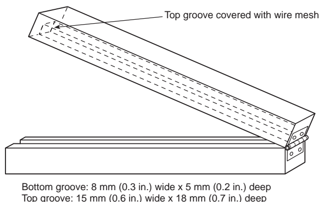
Figure C-1.1 Mounting jig for Test Method 1 specimens.
