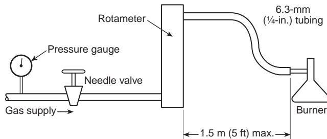
Figure 10-4.3 Gas line feed arrangement to burner.
