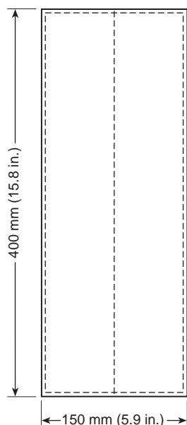
Figure 5-1.1 Multilayer specimen for Test Method 1.
