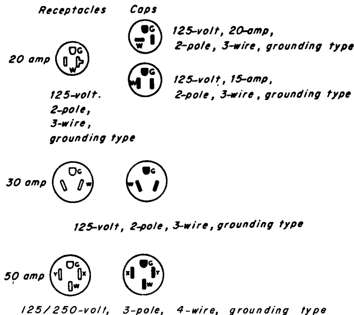
Figure 551-13(c). Configurations for grounding-type receptacles and attachment plug caps used for recreational vehicle supply cords and recreational vehicle lots.
