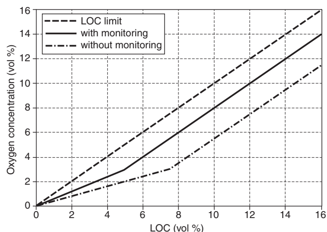
FIGURE A.7.7.2.7 Oxidant Control Limits as a Function of LOC.
