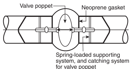
FIGURE A.12.2.2.1 Flow-Actuated Float Valve.
