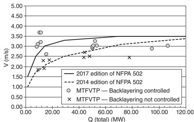
FIGURE D.3.1.2 Critical Velocity Equation from 2014 and 2017 Editions of NFPA 502 Versus MTFVTP.
