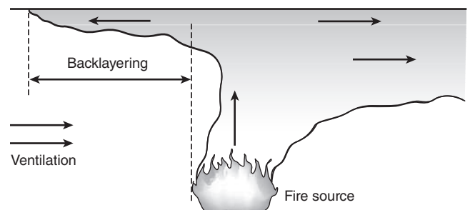
FIGURE A.3.3.5(b) Ventilated Tunnel Fire with Smoke Backlayering Distance Confined.
