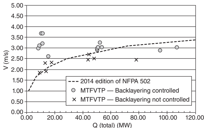
FIGURE D.3.1.1 Critical Velocity Equation from the 2014 Edition of NFPA 502 Versus MTFVTP.
