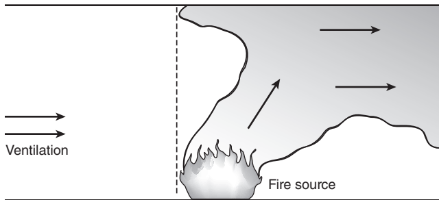
▲ FIGURE A.3.3.5(c) Ventilated Tunnel Fire with Smoke Backlayering Prevented.
