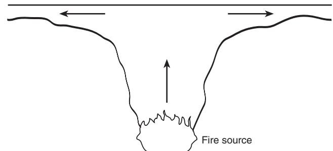
FIGURE A.3.3.5(a) Tunnel Fire Smoke Spread With Insufficient or No Ventilation.
