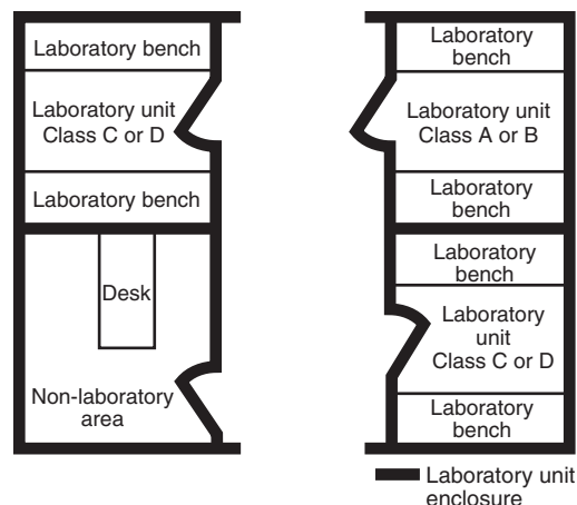
FIGURE D.2.4(e) Separation of Laboratory Units and Non-Laboratory Areas.
