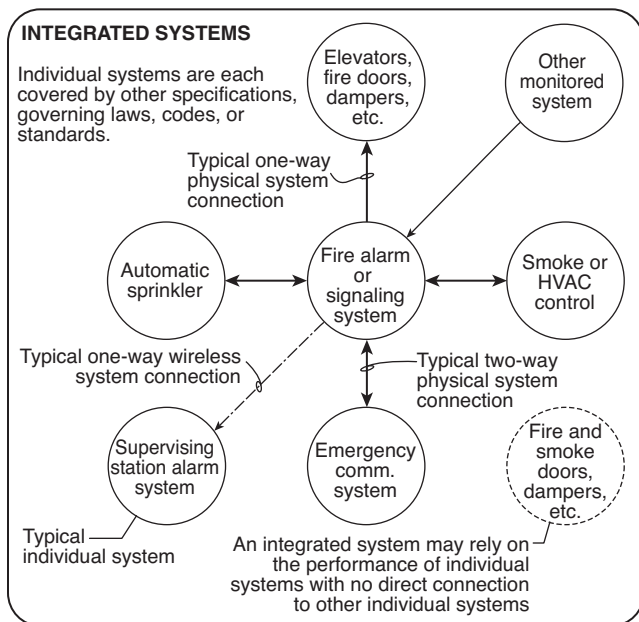
FIGURE A.3.3.25.4 Integrated System. (Source: R.P. Schifiliti Associates, Inc.)
