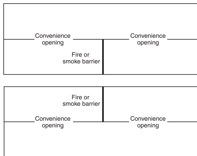
FIGURE A.4.7.2(4) Convenience Opening Arrangement.
