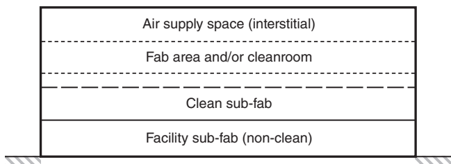
N FIGURE A.3.3.6 Sample Single Cleanroom Production Unit (CPU) Concept.
