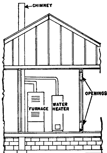
Fig. 1-A. Appliances Located in Confined Spaces All Air from Inside the Building. See 1404 (a).
