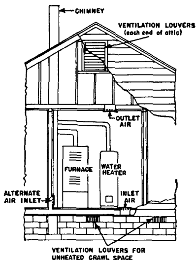
Fig. 1-D. Appliances Located in Confined Spaces All Air from Outdoors — Inlet Air from Ventilated Crawl Space and Outlet Air to Ventilated Attic. See 1404 (b).
