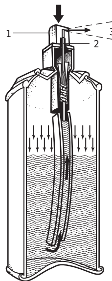
FIGURE A.3.3.2 One Type of Aerosol Container (Cutaway View). When the plunger (1) is pressed, a hole in the valve (2) allows a pressurized mixture of product and propellant (3) to flow through the plunger's exit orifice. [Source: Fire Protection Handbook , 19th edition]
