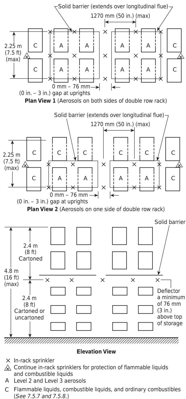
FIGURE 7.5.1 Special Protection for Aerosol Cooking Spray Products and Level 2 and Level 3 Aerosol Products in Double-Row Racks.
