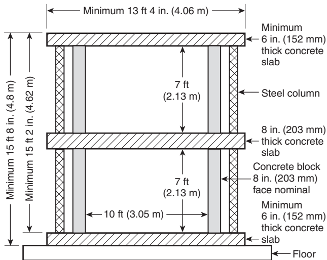
FIGURE 4.2.3 Front View of Test Apparatus Structure (not to scale). For exact dimensions, see 4.2.1 through 4.2.7.
