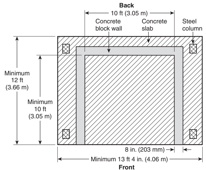
FIGURE A.4.2.3(a) Plan View of Test Apparatus — Both Stories (not to scale).
