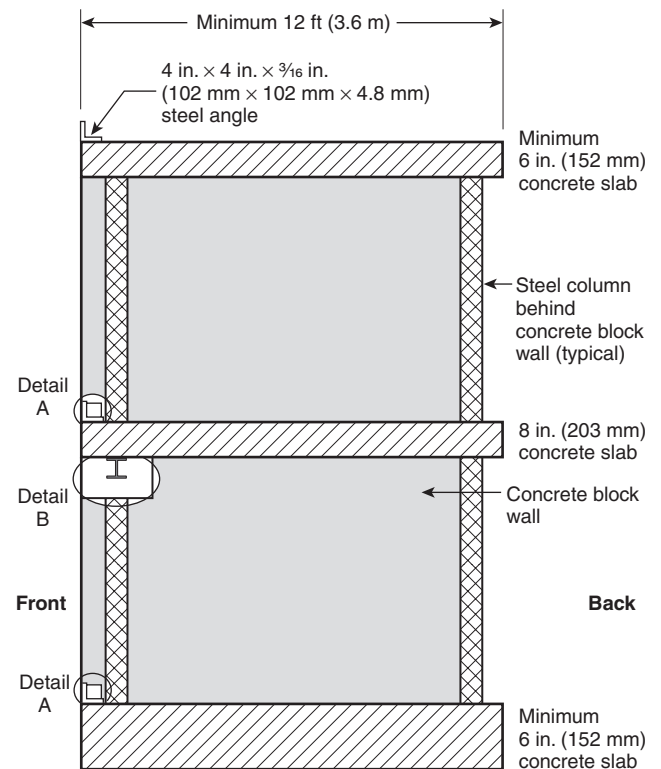
FIGURE A.4.2.3(b) Section View Through Test Apparatus (not to scale). For Details A and B, see Figure A.4.2.3(c).
