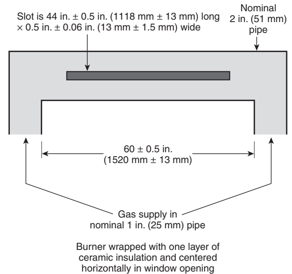
FIGURE 4.4.6 Plan View of Window Burner (not to scale).
