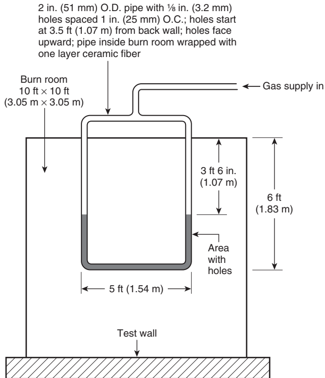
FIGURE 4.4.3.6 Burn Room Burner — Plan View (not to scale).
