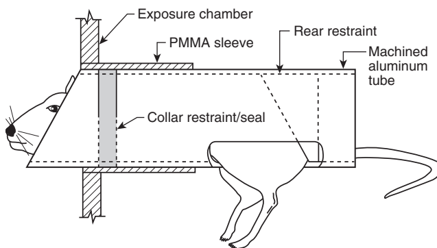
FIGURE A.5.13 Animal Restrainer.
