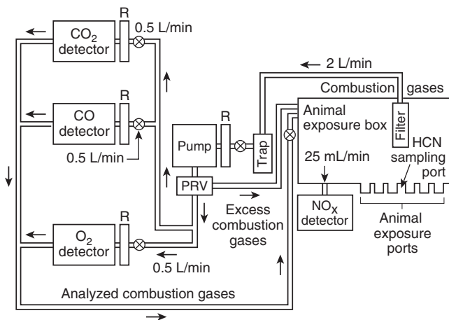
FIGURE 5.11.1 Gas Sampling System.
