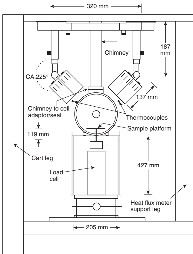
FIGURE 5.4.1(a) End View Showing Dimensions Pertinent to Combustion Cell and Heaters.
