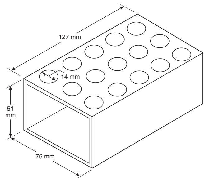
FIGURE 5.5.3.1 Calibration Jig Used for Checking the Uniformity of Irradiance.
